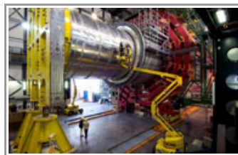
Insertion of the inner vacuum tank.
