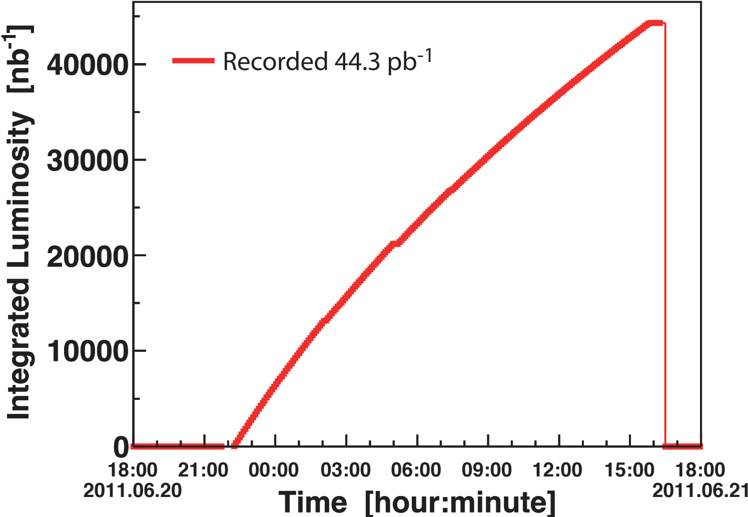
CMS Integrated luminosity 20th June 2011
