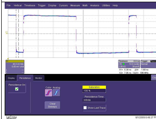
gbtia OUTN with User pattern (200 Mbit/s) DC current = 0 mA
