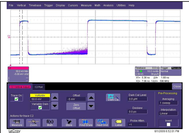
gbtia OUTP with User pattern (200 Mbit/s) DC current = 0.92 mA
