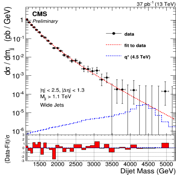
Figure 3: Di-jet invariant mass spectrum, showing the expected signal distribution from a hypothetical particle with 4.5 TeV transforming into two jets
