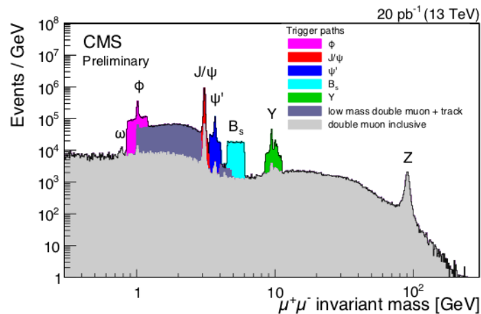
Figure 2: The di-muon invariant mass spectrum at 13 TeV
