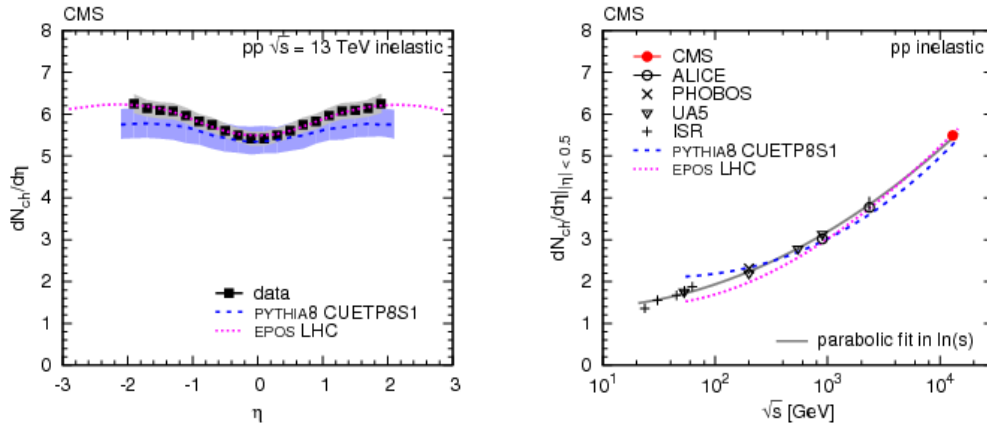
Figure 1: Measured charged-hadron production as a function of pseudorapidity (left), and the multiplicity in the central region compared to previous measurements at lower energies and theoretical models.
